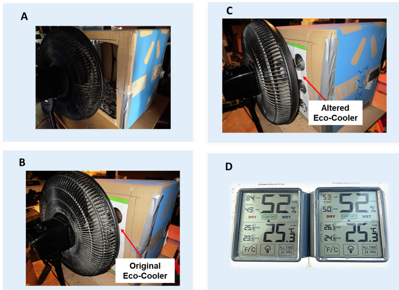
Figure 3. Experimental scenarios and equipment. Three cooling apparatus scenarios were created for testing. A) In Scenario 1, only a fan blew air directly into the cardboard box. B) In Scenario 2, a fan blew air through the original Eco-Cooler into the cardboard box. C) In Scenario 3, the fan blew air through the altered Eco-Cooler into the cardboard box. D) Two digital thermometers were used to collect data. Temperatures were measured under control conditions and with the original or altered Eco-Cooler. Each scenario was tested under similar conditions.
